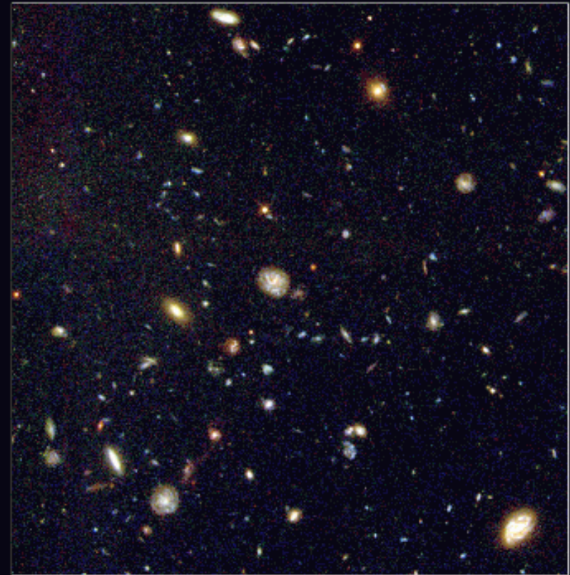
Hubble Deep Field South Hubble Space Telescope • WFPC2
