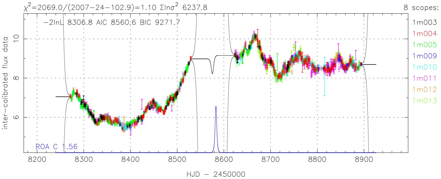
DREAM fit to F9 data B
