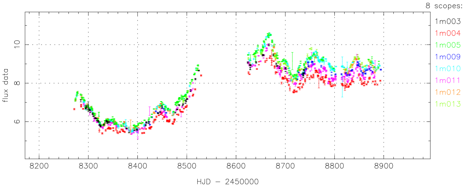
DREAM fit to F9 data B
