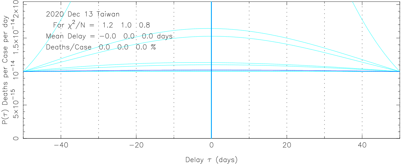
COVID-19 Delay Distribution (Deaths per Case per Day) Taiwan MEME fit to COVID-19 data from ECDC 2020 Dec 13
