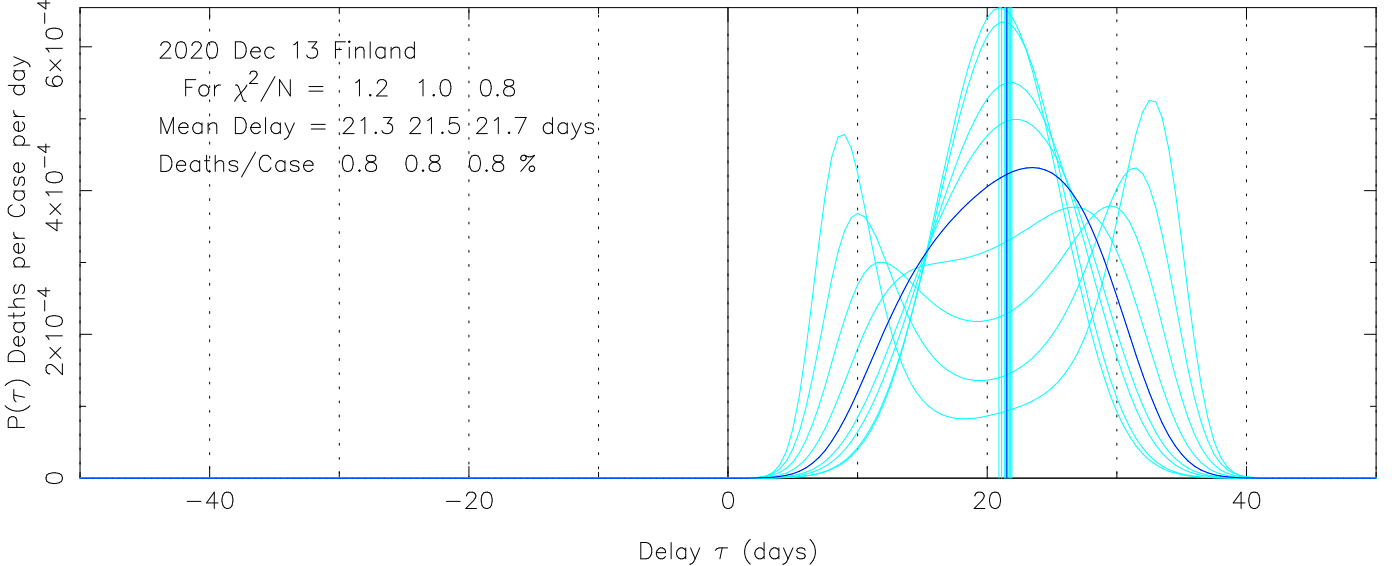
COVID-19 Delay Distribution (Deaths per Case per Day) Finland MEME fit to COVID-19 data from ECDC 2020 Dec 13
