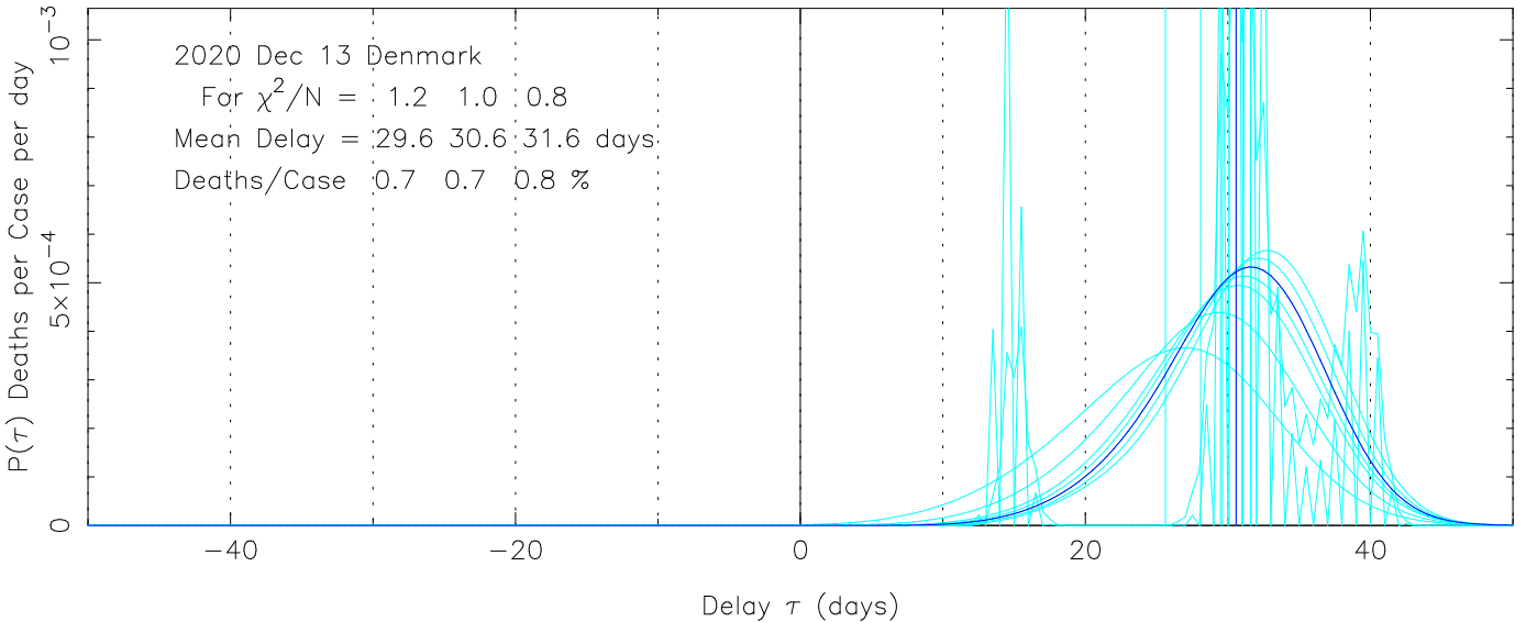
COVID-19 Delay Distribution (Deaths per Case per Day) Denmark MEME fit to COVID-19 data from ECDC 2020 Dec 13
