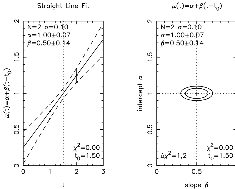
Figure 14: A straight line fits 2 data points exactly.
