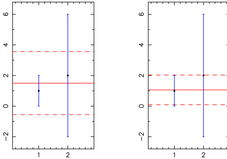
Figure 11: Normal and optimal averages of 2 data points. The normal average gives equal weight to all data points. In this example the normal average is less accurate than the first data point alone. The optimal average uses inverse-variance weights, 1/\sigma^2 , and is always more accurate than every individual data point.
