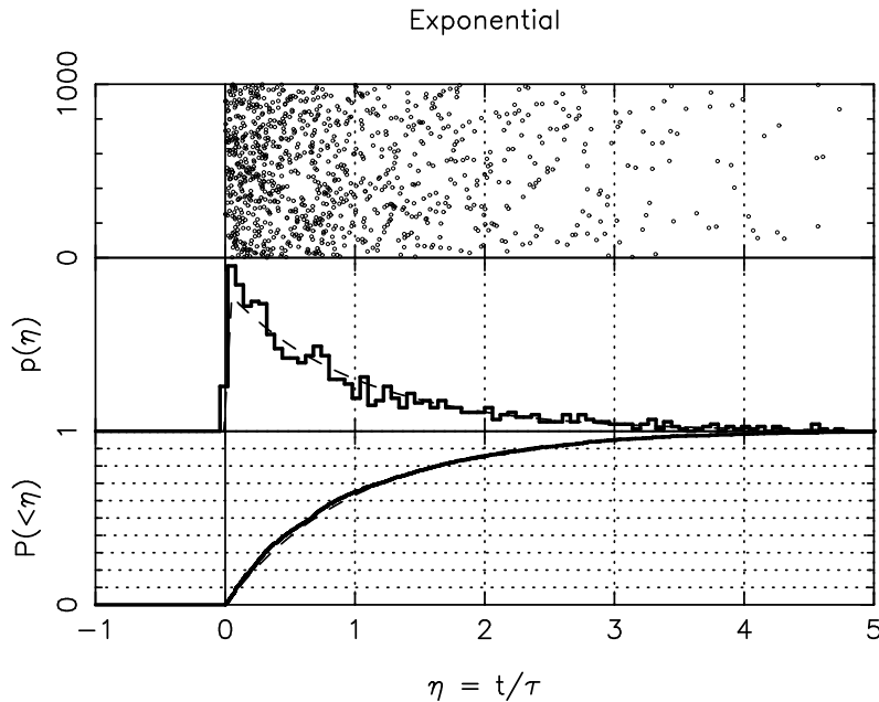
Figure 8: Exponential random numbers with an e-folding time \tau = 1 . The 1000 random numbers (top panel) are binned (middle panel) for comparison with the probability map. This is then integrated (lower panel) for comparison with the cumulative probability.
