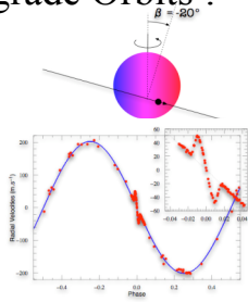
Radial velocity vs orbital phase.
